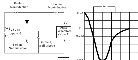
FIG.5-TEST CIRCUIT DIAGRAM AND REVERSE RECOVERY TIME CHARACTERSITIC
