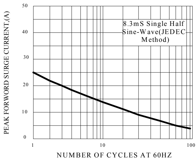
FIG.3-MAXIMUN NON-REPEITIVE FORWARD SURGE CURRENT
