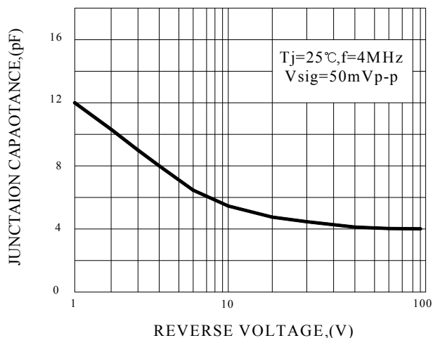
FIG.6-TYPIAL JUNCTION CAPAOTANCE
